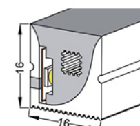
MOD. V040 16x16 mm PCB 10 mm
