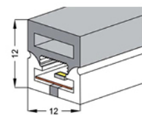
MOD. H006 12x12 mm PCB 8 mm
