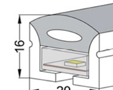
MOD. H010 20x16 mm PCB 10 mm
