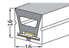
MOD. H008 16x16 mm PCB 12 mm
