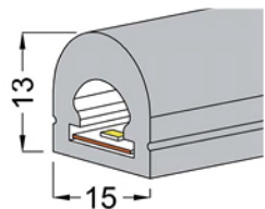
MOD. R021 13x15 mm PCB 10 mm
