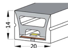
MOD. H041 20x14 mm PCB 12 mm
