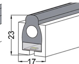
MOD. H051 17x23 mm PCB 10 mm
