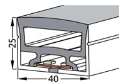
MOD. H047 40x25 mm PCB 20 mm
