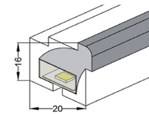
MOD. H049 16x20 mm PCB 10 mm
