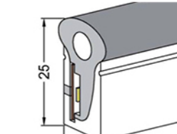
MOD. V019 12x25 mm PCB 12 mm
