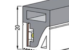
MOD. V025 12x20 mm PCB 10 mm
