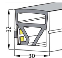
MOD. V028 30x32 mm PCB 15 mm
