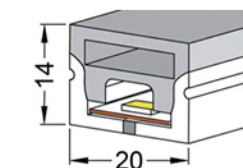
MOD. H007 20x14 mm PCB 12 mm
