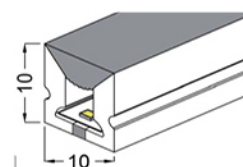
MOD. H004 10x10 mm PCB 6 mm
