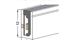
MOD. V015 12x20 mm PCB 10 mm
