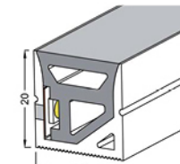
MOD. V043 20x20 mm PCB 10 mm
