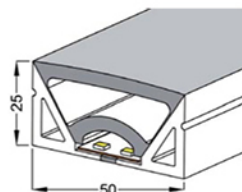
MOD. H048 50x25 mm PCB 20 mm
