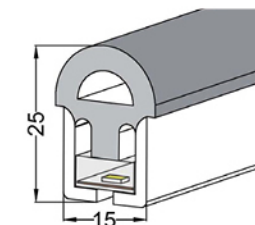
MOD. H050 15x25 mm PCB 10 mm
