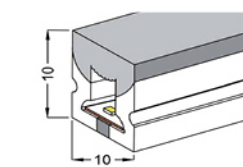
MOD. H005 10x10 mm PCB 6 mm
