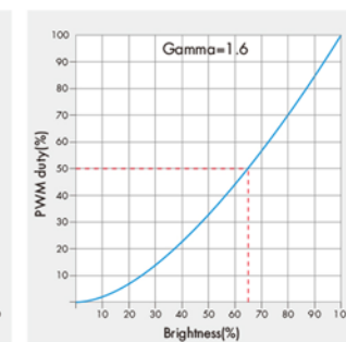
Dimming curve for RGB/DIM
